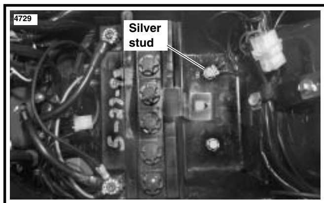
Figure 18. Main Circuit Breaker Silver Stud
