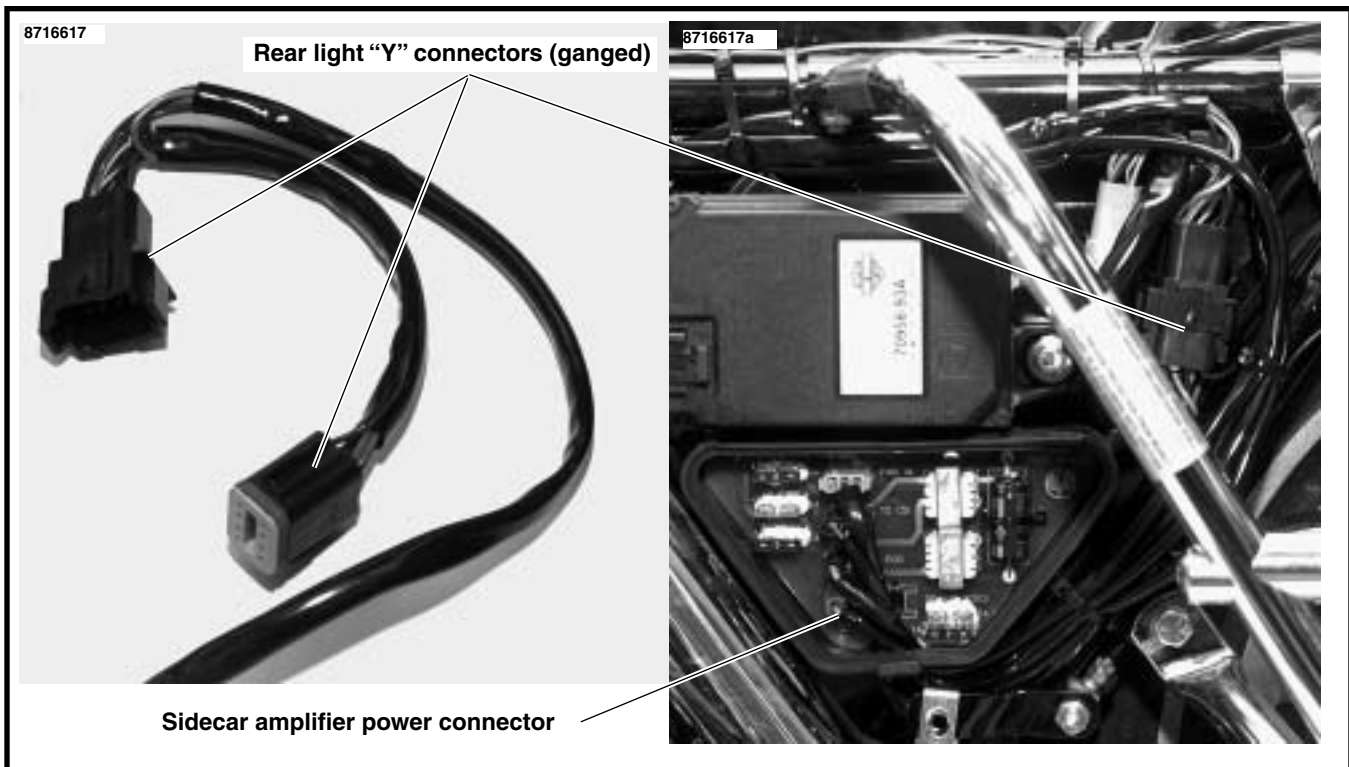
Figure 20. 1994 Sidecar/Motorcycle Rear Light Harness
