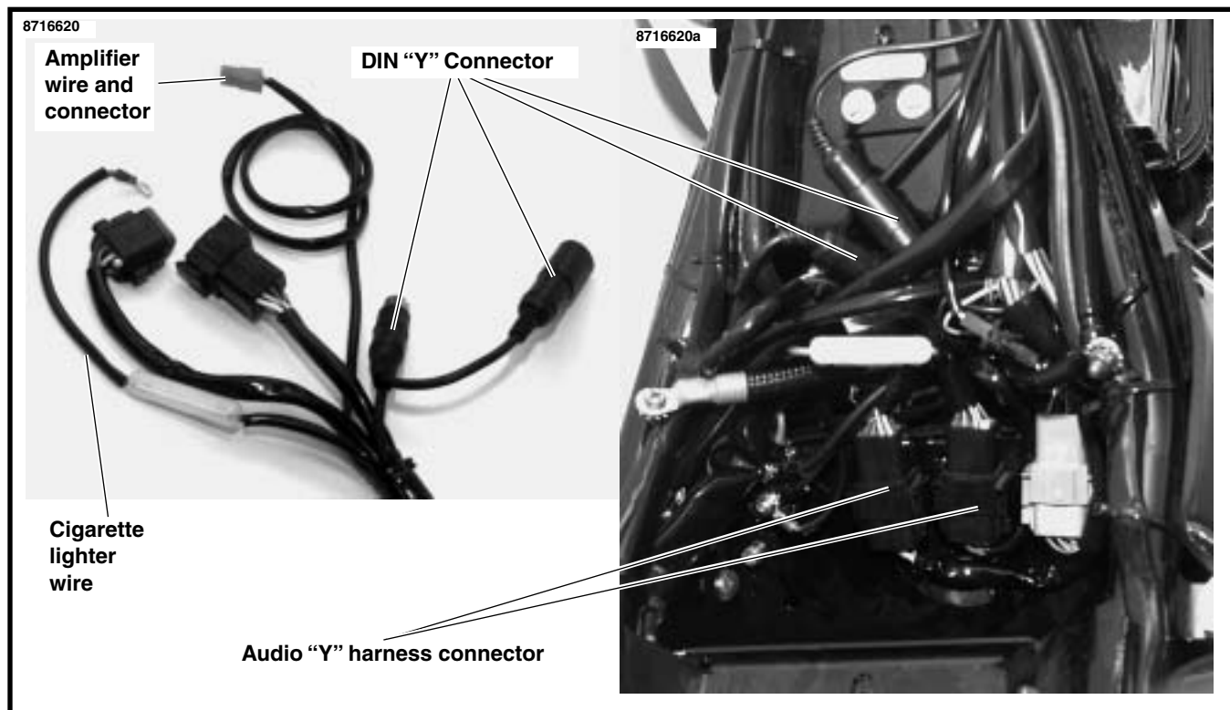
Figure 22. 1994 Sidecar Audio Harness
