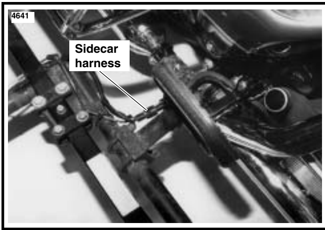
Figure 15. Sidecar Harness - 1992 and Earlier
