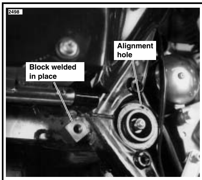
Figure 7. Frame Mounting Block Welding
