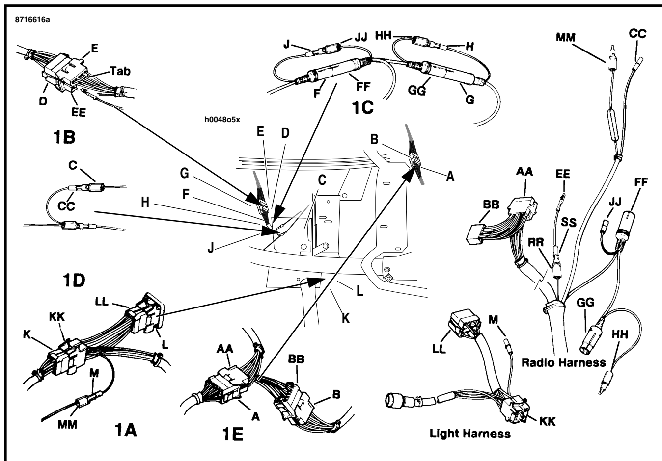
Figure 14. Tie Ultra Wiring Harness - 1989 to 1990
