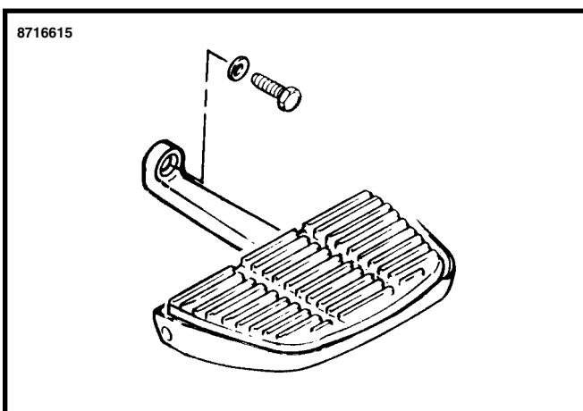
Figure 11. Right Passenger Footboard Motorcycle and Mounting
