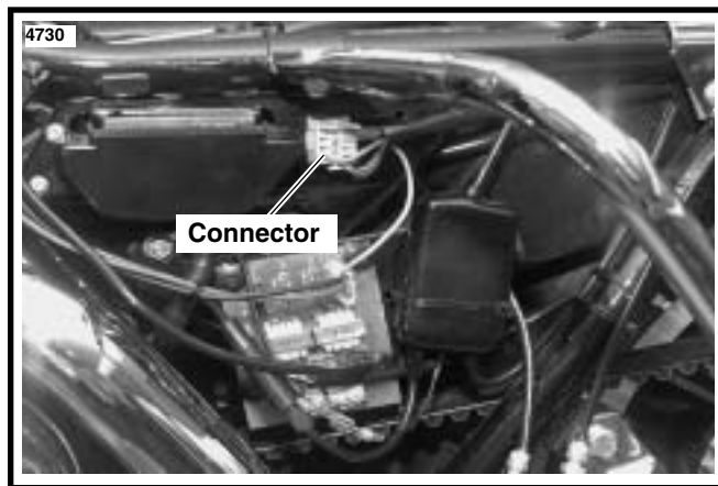
Figure 12. 1992 and Earlier Connector Location (Left Side Cover Removed)
