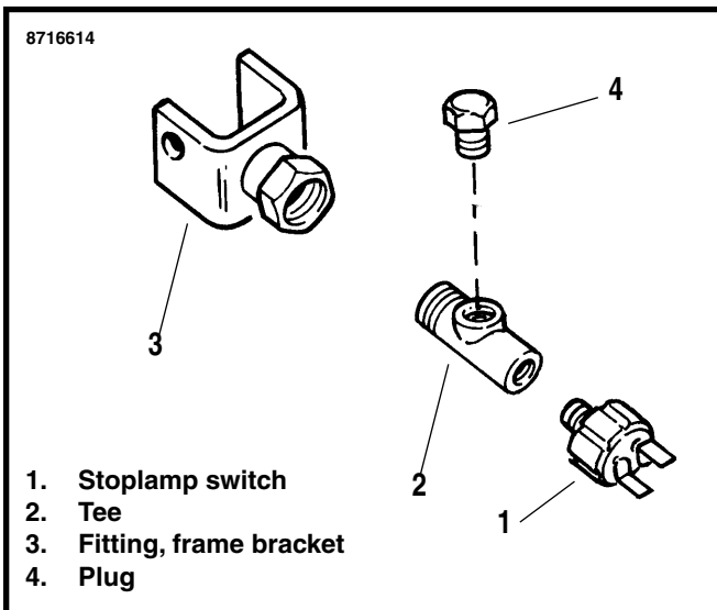
Figure 10. Sidecar Brake Line Connection - 1992 and Later
