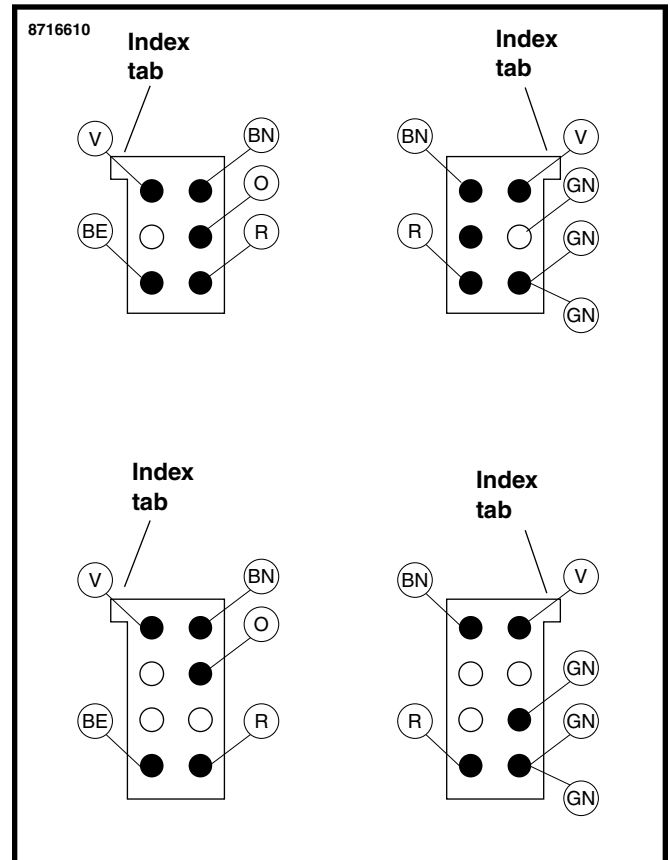
Figure 13. Converting 6 Pin Connectors to 8 Pin Connectors
