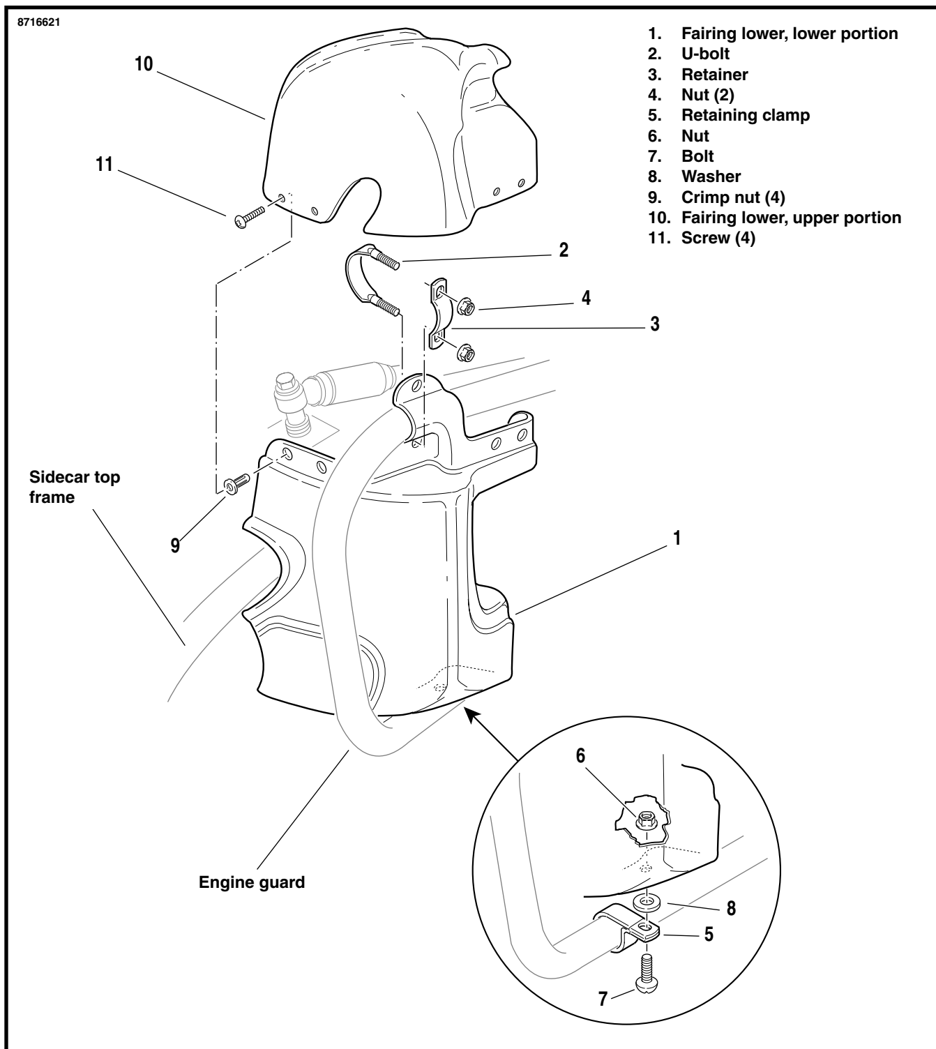
Figure 23. FLHTC Sidecar Fairing Lower
