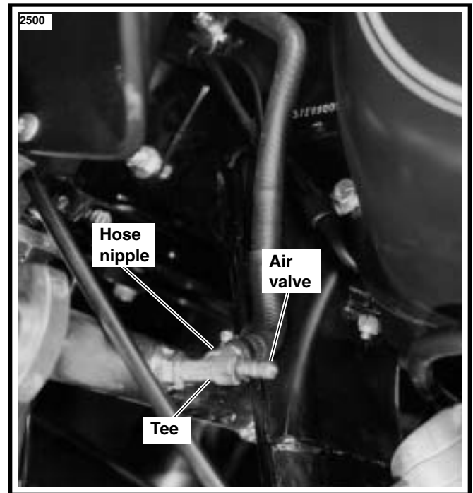
Figure 2. Rerouted Air Suspension Valve
