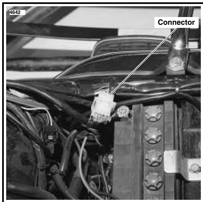
Figure 17. Connecting Sidecar Harness - 1993 Shown
