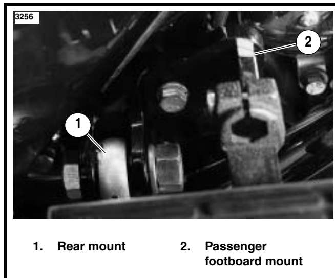
Figure 8. Rear Mount Installed
