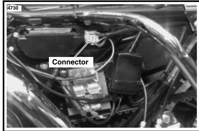
Figure 16. 1992 and Earlier Connector Location (Left Side Cover Removed)
