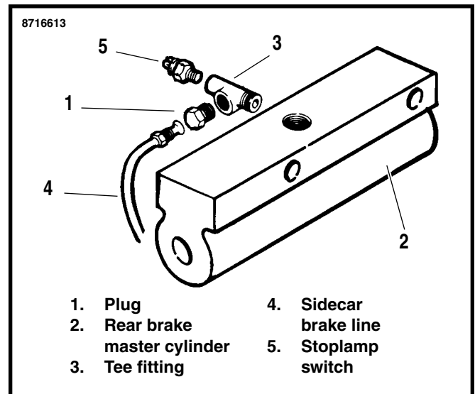
Figure 9. Sidecar Brake Line Connection - 1991 and Earlier
