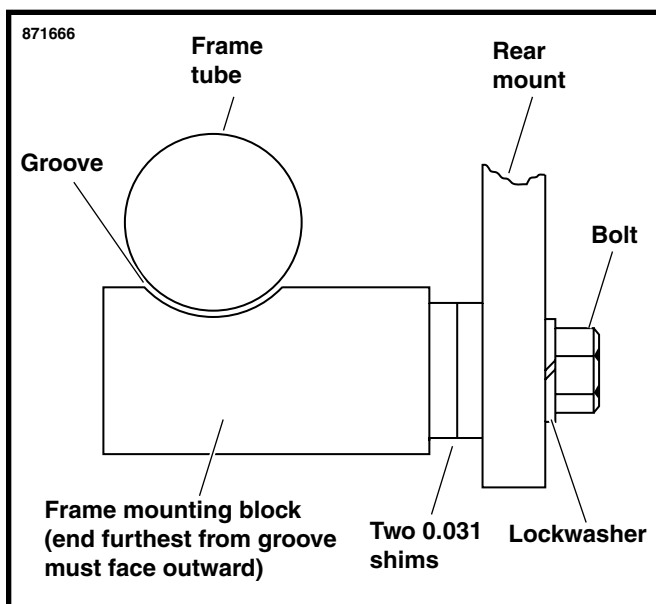
Figure 6. Positioning Mounting Block
